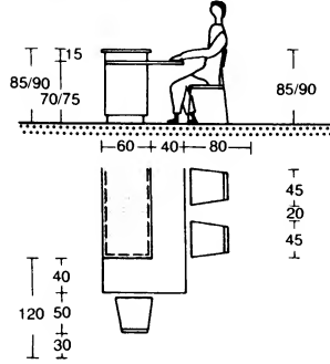
⑤ Fitted table
